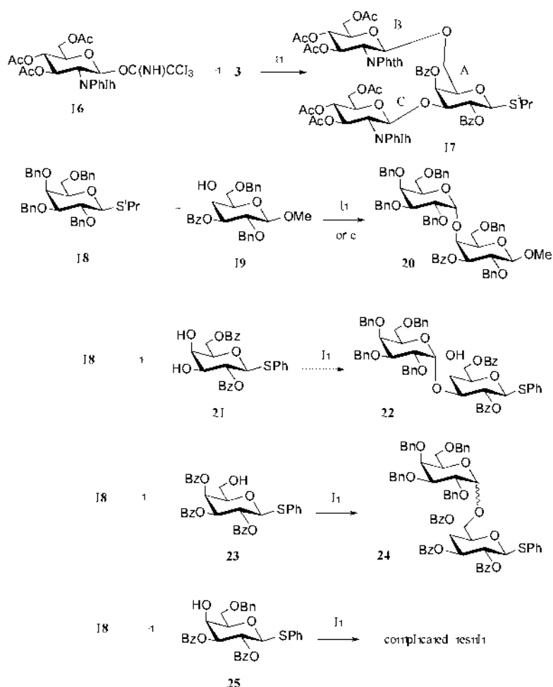
Scheme 2 Reagents and conditions (yields): a) TMSOTf, CH 2 Cl 2 (54%); b) NIS, TMSOTf, Et 2 O (80% for 20 , 62% for 22 , 96% for 24 ); c) MeOTf, CH 2 Cl 2 (56–70%).
