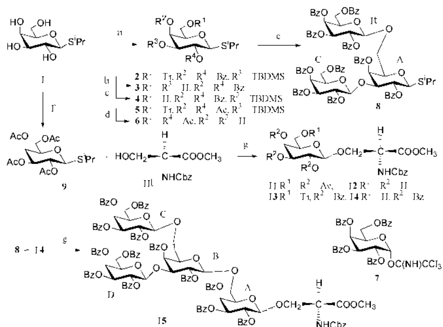
Scheme 1 Reagents and conditions (yields): a) TrCl, pyridine; TBDMSCl, imidazole; BzCl (76%); b) 90% TFA (80%); c) Method A: FeCl 3 ·6H 2 O (50%); Method B: 50% TFA (86.3%); d) 90% TFA (85%); e) TMSOTf (90%); f) Ac 2 O, pyridine (100%); g) NIS, TMSOTf (87% for 11 , 91% for 15 ).
